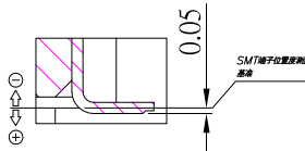
DETAIL A SCALE 16:1
