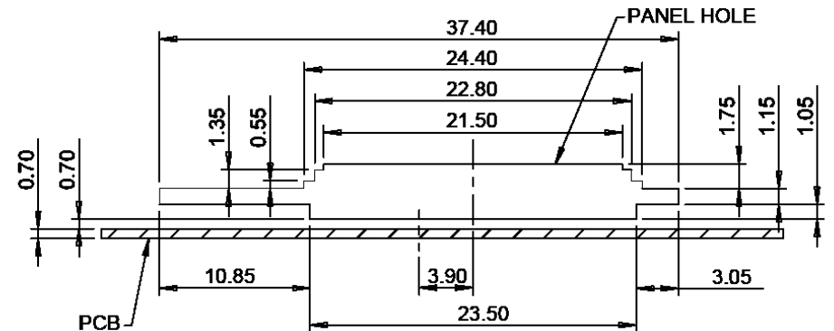
RECOMMEND PANEL HOLE
