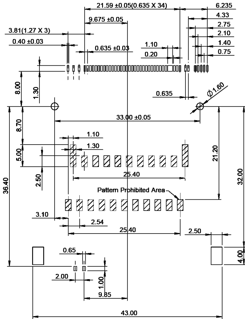
RECOMMEND PCB LAYOUT
