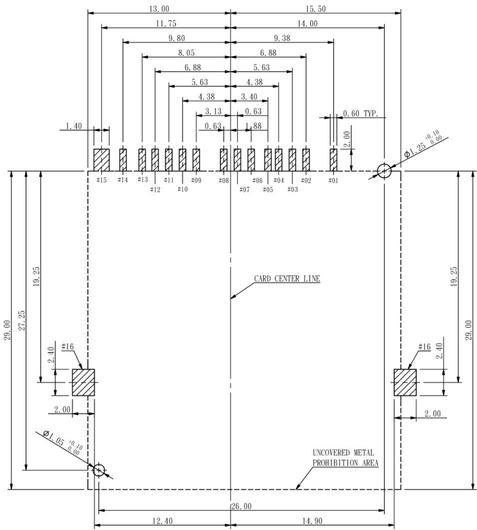
RECOMMEND P. C. B. LAYOUT TOLERANCE \pm 0.05
