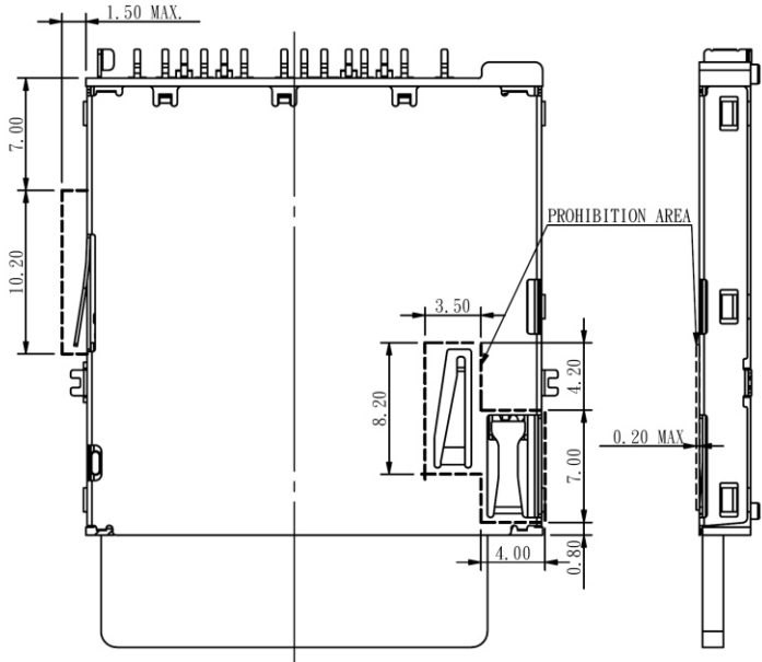
A SIZE WHEN A HOOK PART OPERATES (MAX. 1.5mm)
