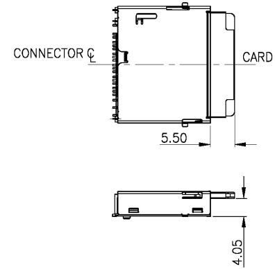
RS MMC/RS MMC 4.0 Card Insert
