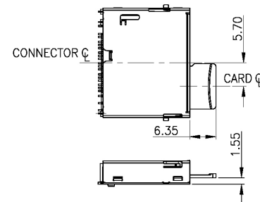
Micro SD Card Insert
