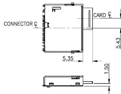
MMC Micro Card Insert
