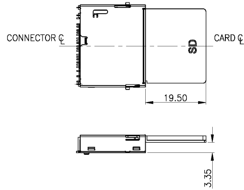
SD Card Insert
