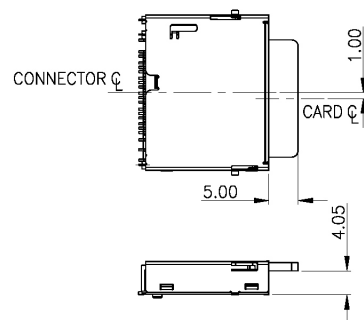
MMC Micro Card Insert
