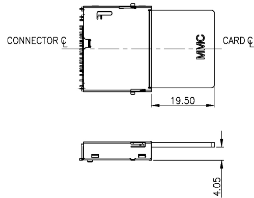
MMC/MMC 4.0 Card Insert
