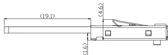
MMC Card Or MMC 4.0 Card Insert Drawing:
