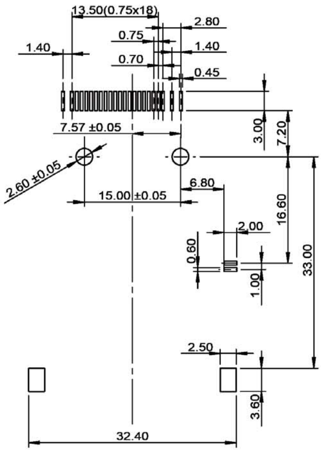
PCB LAYOUT
