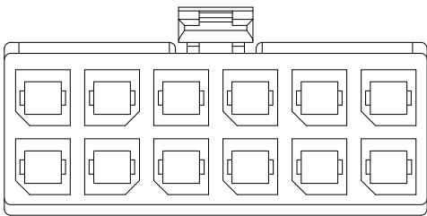
2X6 PIN
