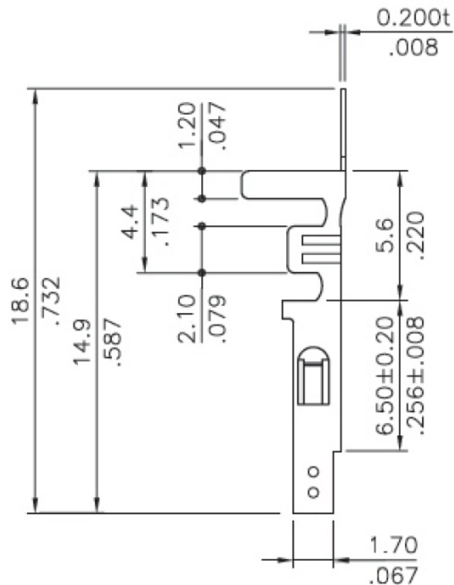
Back View
