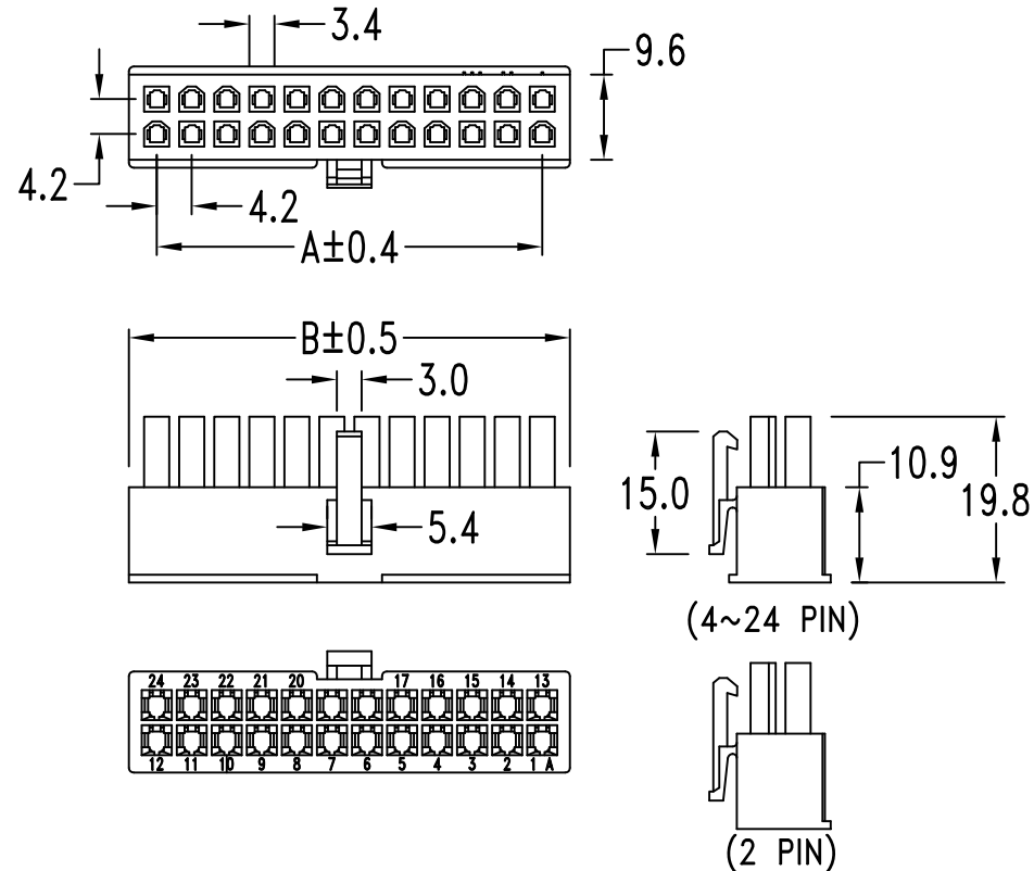
Dimensional Information ( mm )
