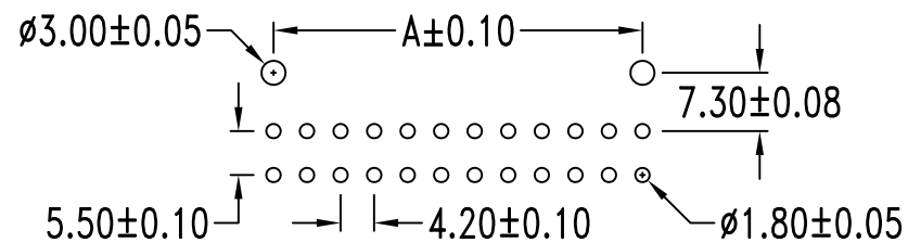
PCB LAYOUT: COMPONENT SIDE
