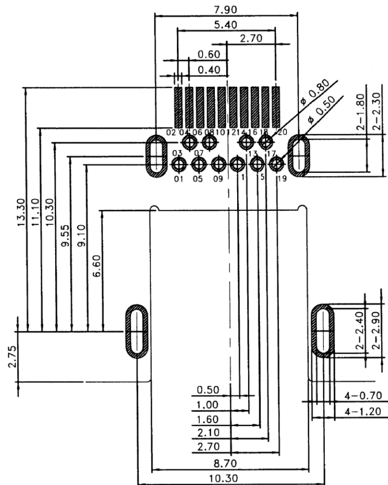
RECOMMENDED. P.C.B LAYOUT TOLERANCERS: \pm 0.02\text{mm}
