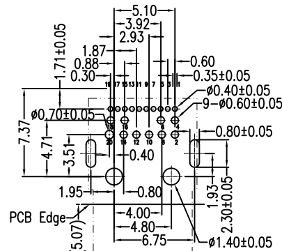
P.C.B Layout t=1.60mm
