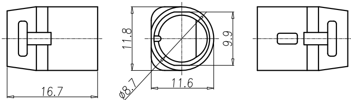
PLASTIC TUBE
