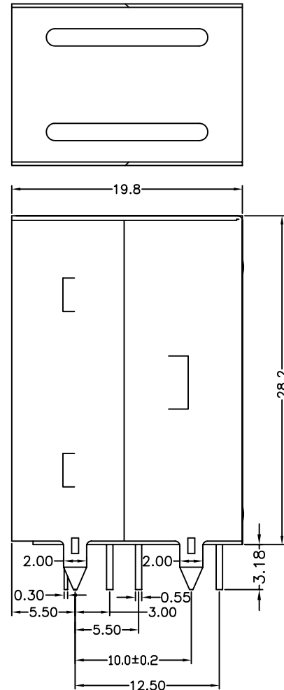
SIDE VIEW
