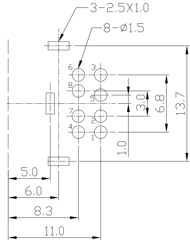
P.C.B LAYOUT ( \pm 0.1 ) (BOTTOM VIEW)
