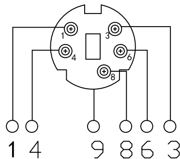
SCHEMATIC DIAGRAM
