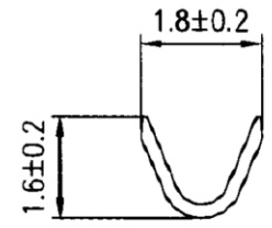
B-B SECTION
