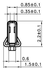
SEC.C-C
