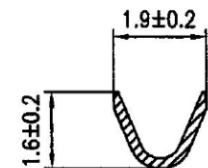
B-B SECTION
