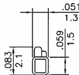
C-C SECTION
