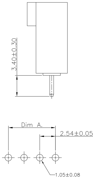
PCB LAYOUT
