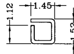
Section C-C
