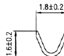
B-B SECTION
