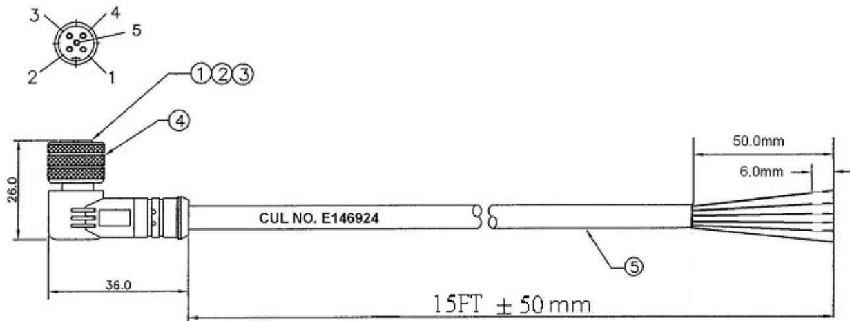
M12-5P-FEMALE
