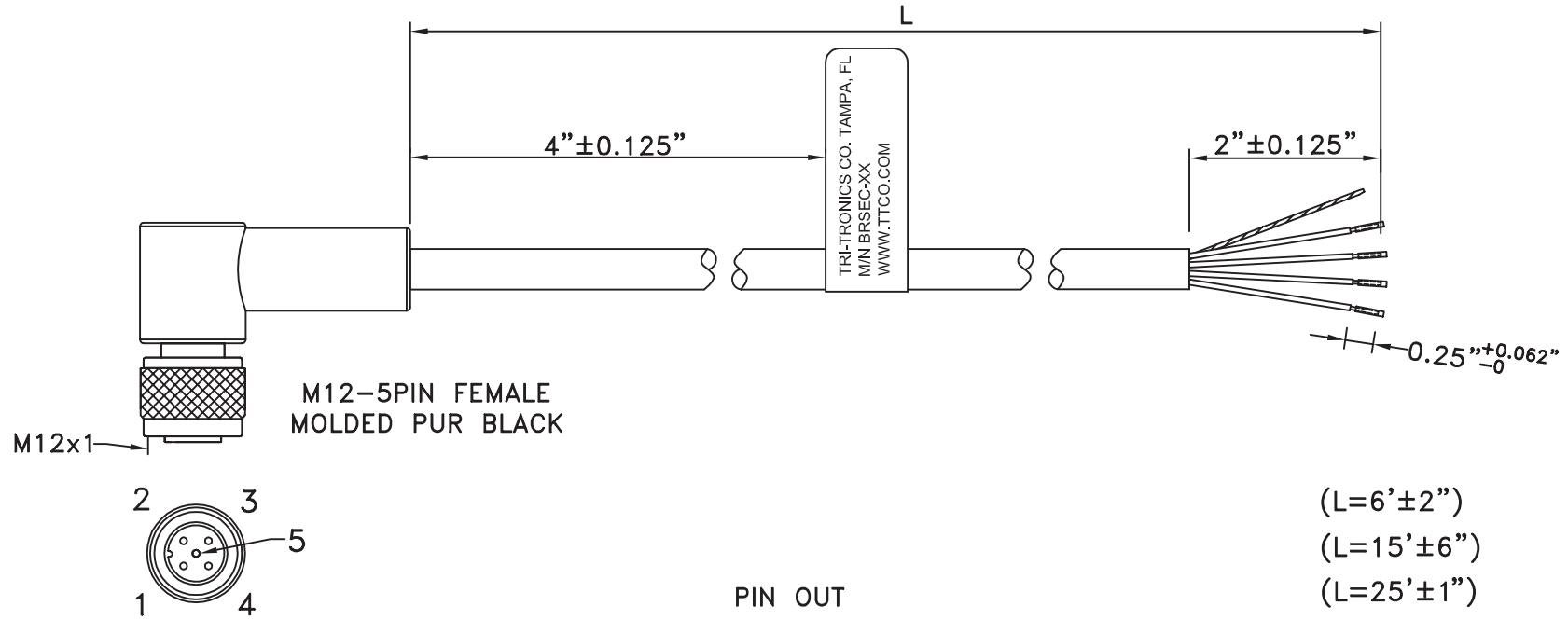
FRONT VIEW
