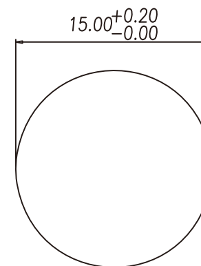
PANEL CUT-OUT
