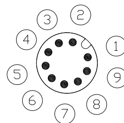
Pin Assignment Front View Scale 2:1
