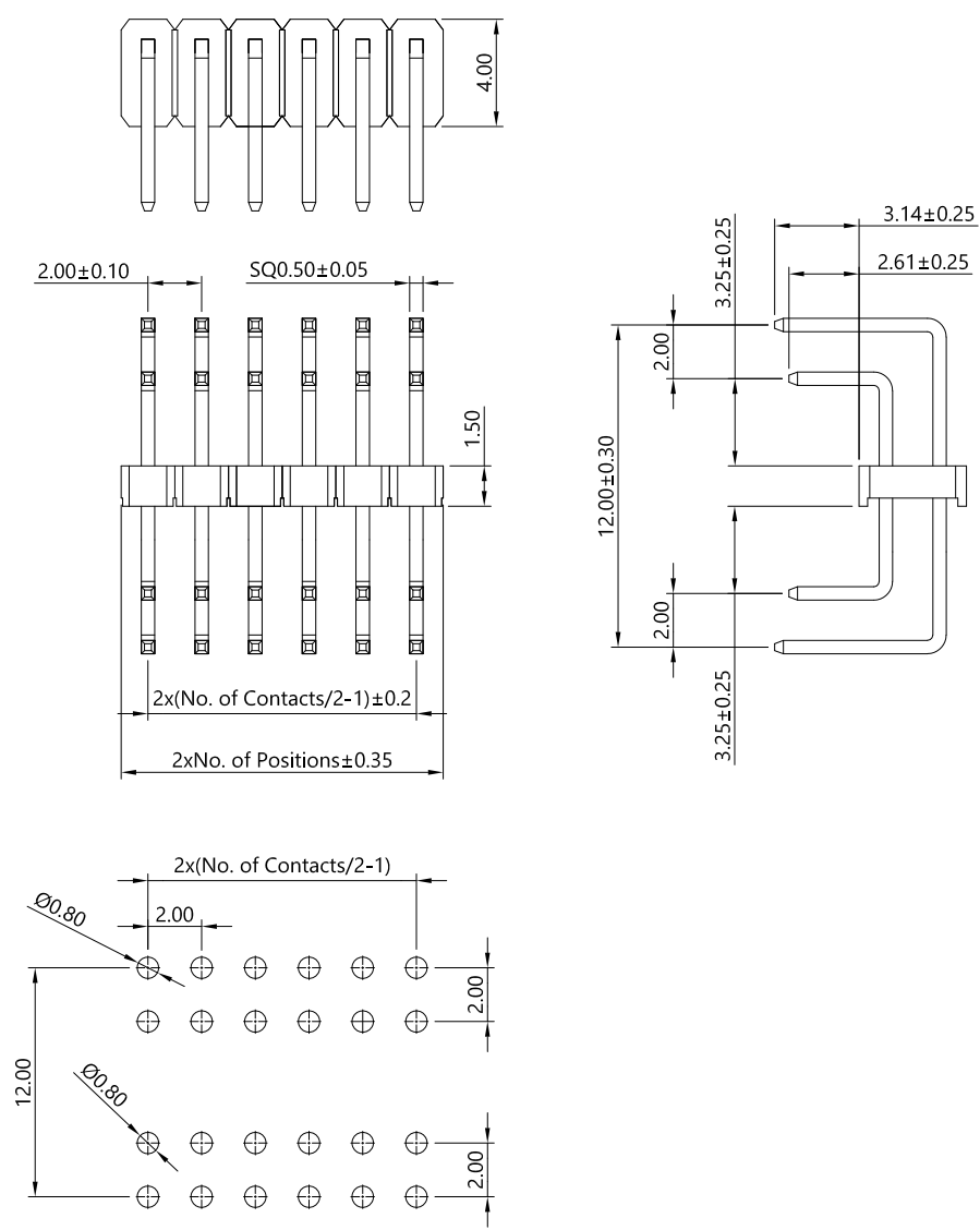
Recommended PCB Layout (PCB Board Tolerance ± 0.05)
