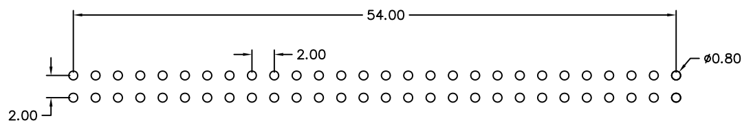
Recommended P.C.B Layout
