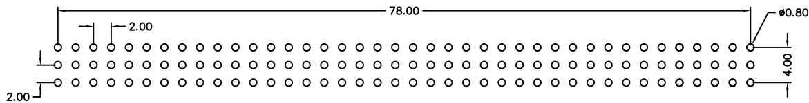
Recommended P.C.B Layout
