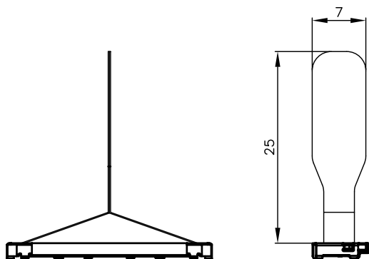
PULL TAB INSTALLATION CONDITION(2:1)
