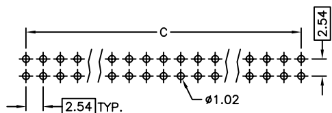
RECOMMEND P.C.B. LAYOUT BOTTOM VIEW
