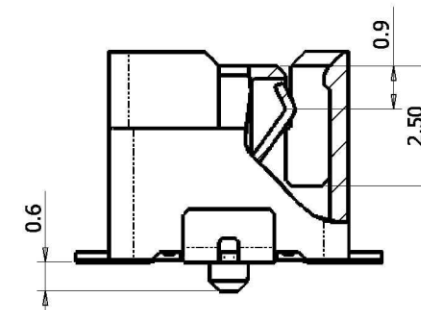
Contact area detail
