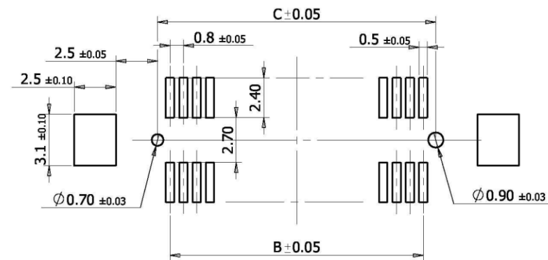
P.C.B Pattern (REF.) component side
