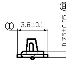
SEC. C-C
