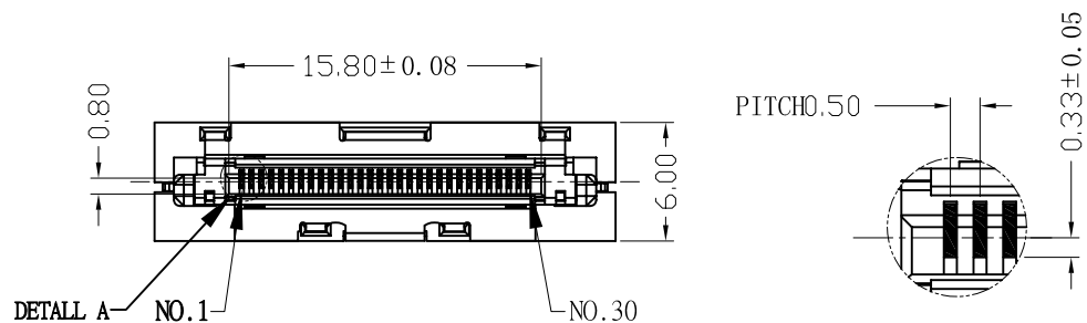
DETAIL A SCALE 5:1
