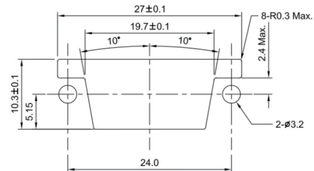
Panel cutout Recommended thickness of panel : 1±0.1
