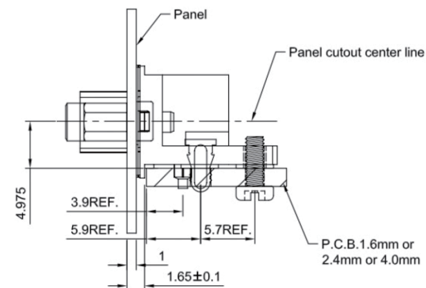
Recommended panel cutout position.
