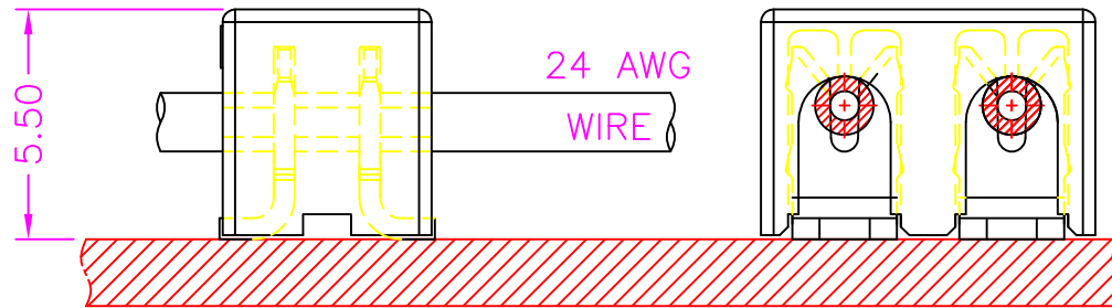
ASSEMBLY LAYOUT
