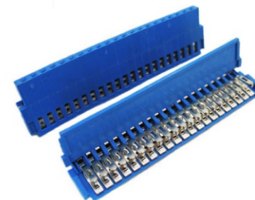
2.54mm PVF-HI-1Xxx
