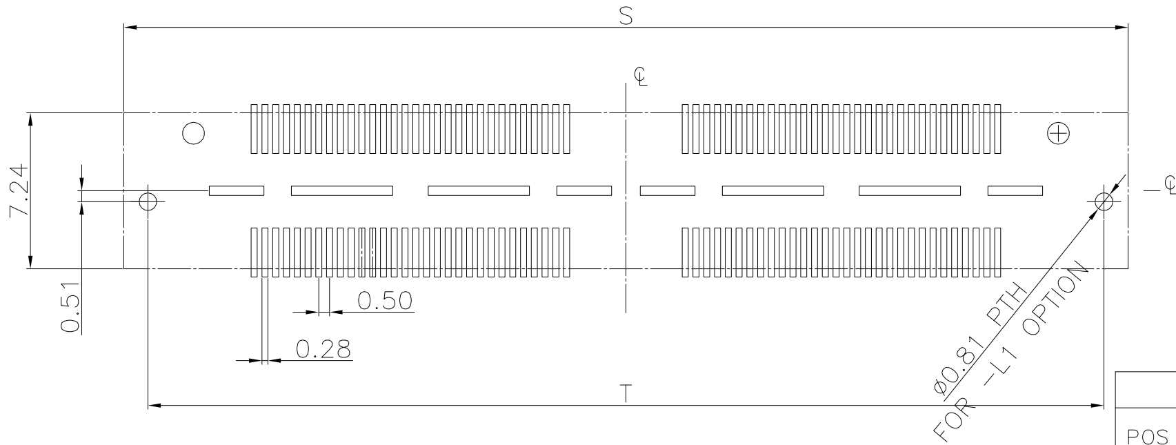
P.C.Board Layout (Tolerance:±0.05)
