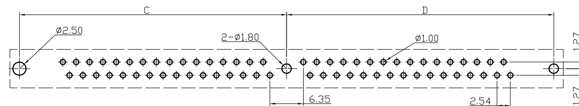
TOP VIEW PCB LAYOUT RECOMMENDED
