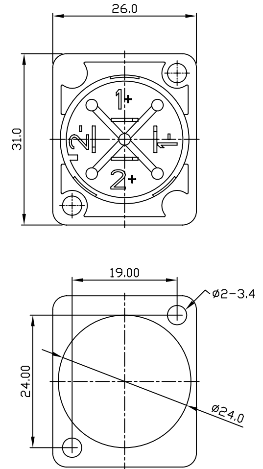
PANEL CUTOUT REAR SIDE(±0.1)
