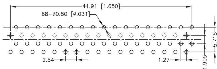
RECOMMENDED P.C.B LAYOUT TOLERANCE ±0.05 TOP VIEW
