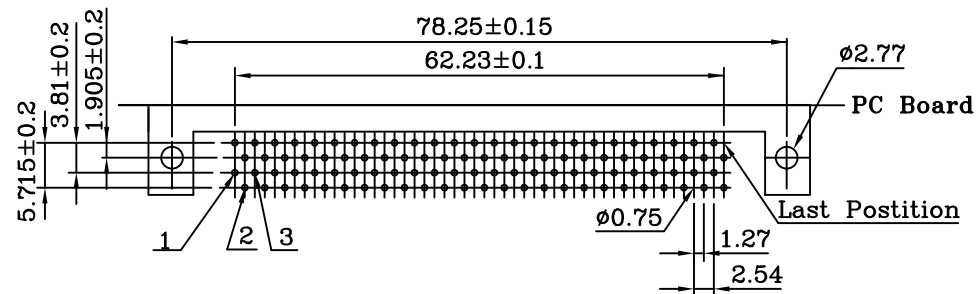
PC Board Mounting Dimensions
