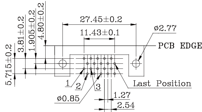
PCB Layout
