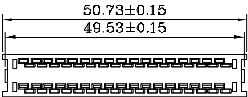
Termination Cover (1 Places)
