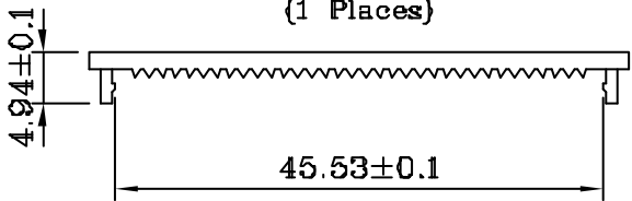
Termination Cover (1 Places)
