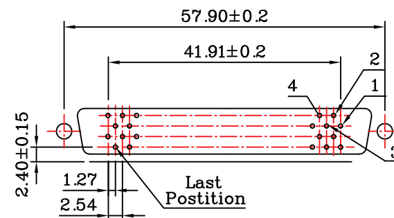
L2:Standard PCB LAYOUT
