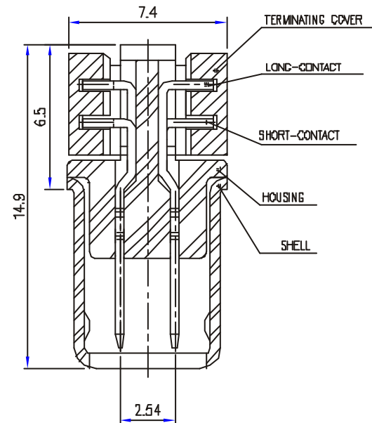
SECTION A-A SCALE 5:1
