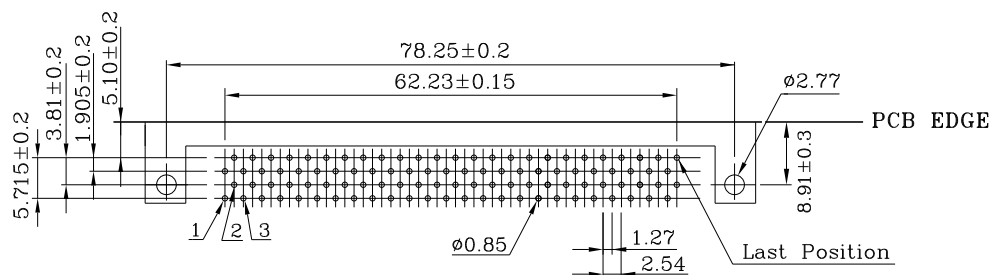
PCB Layout
