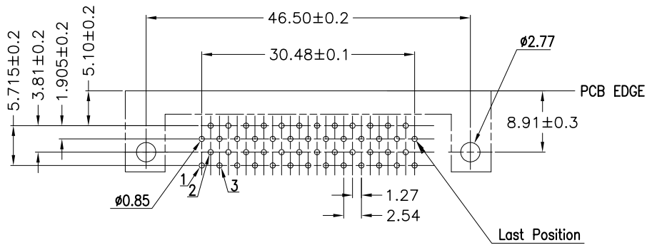
PCB Layout
