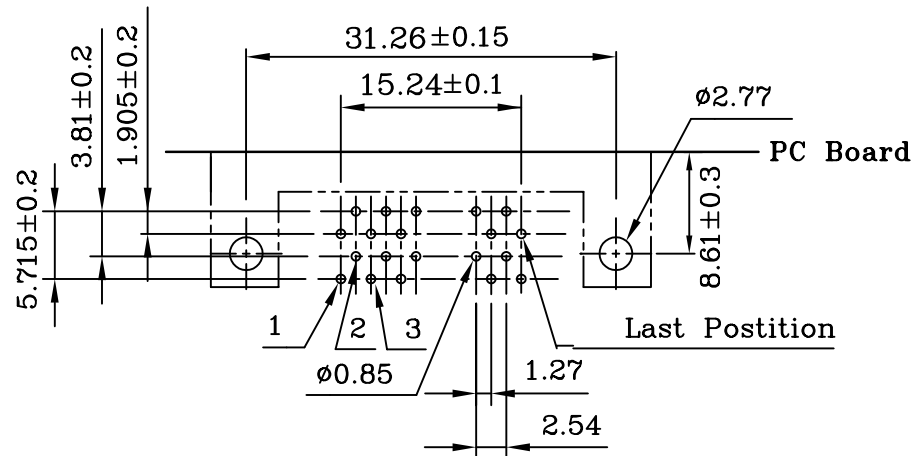
PC Board Mounting Dimensions
